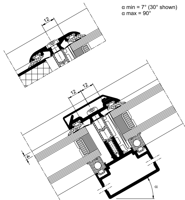
PURLIN
