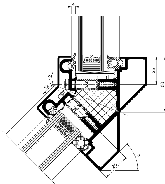
SLOPE/VERTICAL CONNECTION
