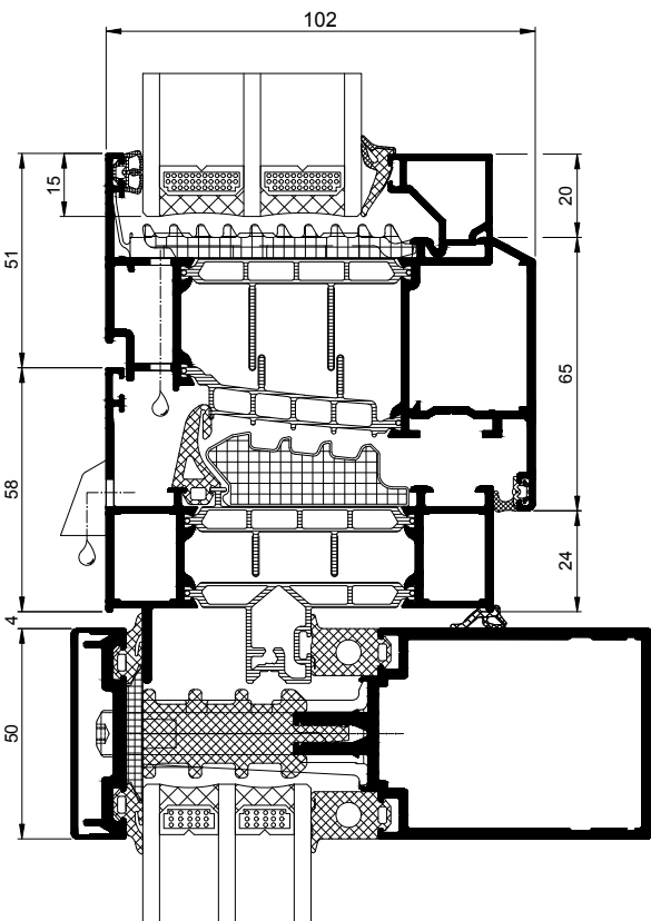
Curtain Wall Viewed Externally CRO-133
